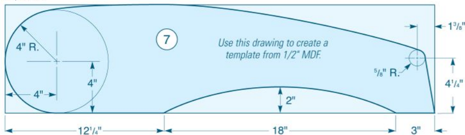
Seat (Top View)
