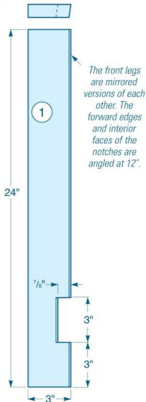
Front Leg (Top and Side Views)
