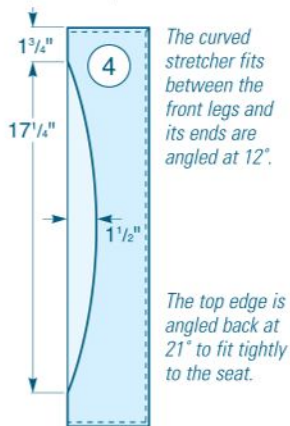
Curved Stretcher (Front View)
