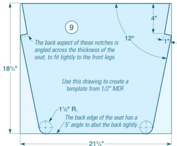
Seat (Top View)
