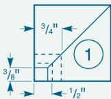
Leg Mortise and Tenon Locations (Front and Top Views)
