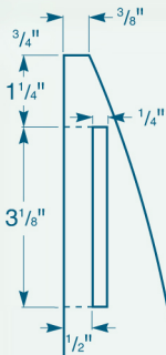
Leg Mortise and Tenon Locations (Front and Top Views)
