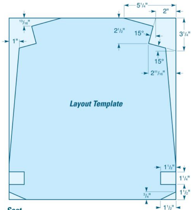
Seat (Top View)
