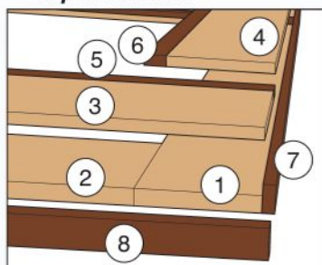
Lap Joint Detail
