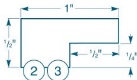
Frame (End View)
