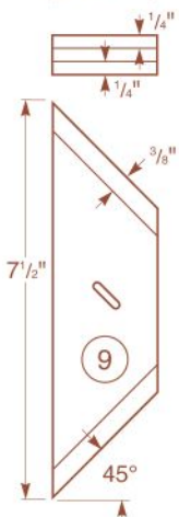
Corner Block (Top View)
