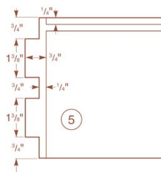
Apron Tenon (Inside View)
