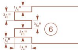
Bottom Stretcher (Top View)
