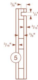
Apron (End View)
