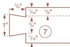
Bottom Stretcher (Top View)
