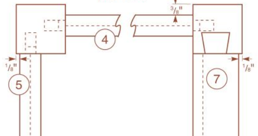
Apron Offsets (Top View)
