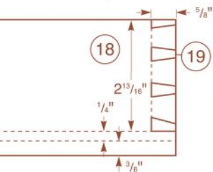
Drawer Back (Side View)
