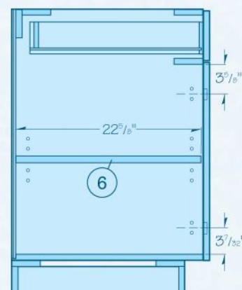
Carcass and Base Elevation (Section View)
