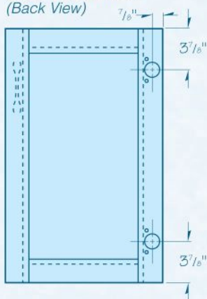
Door Elevation (Back View)
