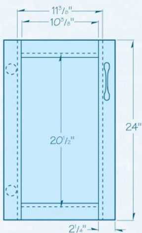
Door Elevation (Front View)
