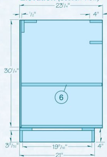
Carcass and Base Elevation (Section View)
